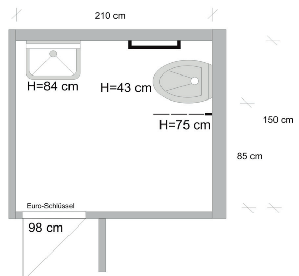
WC and WC layout plan
